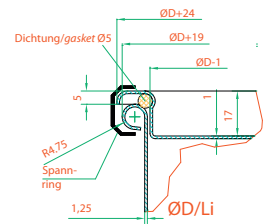
Deckel, Zarge und Spannring /cover, jacket and clamping ring
